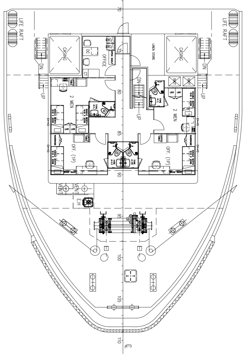
UPPER FORECASTLE DECK
