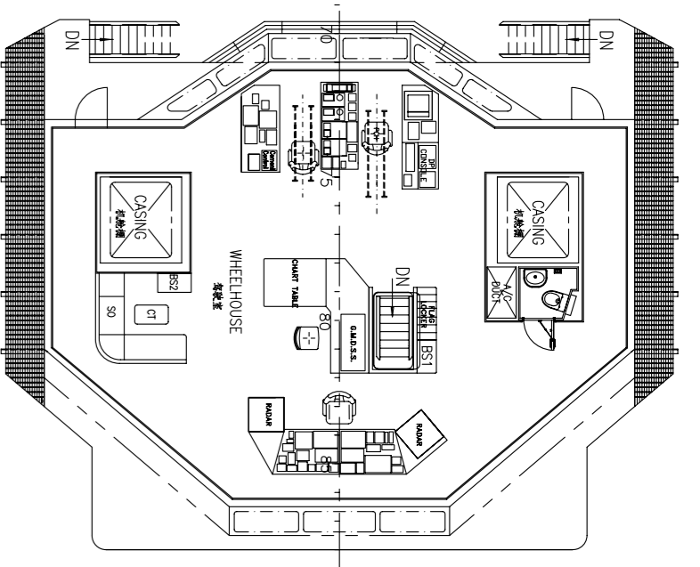
BRIDGE DECK PLAN
