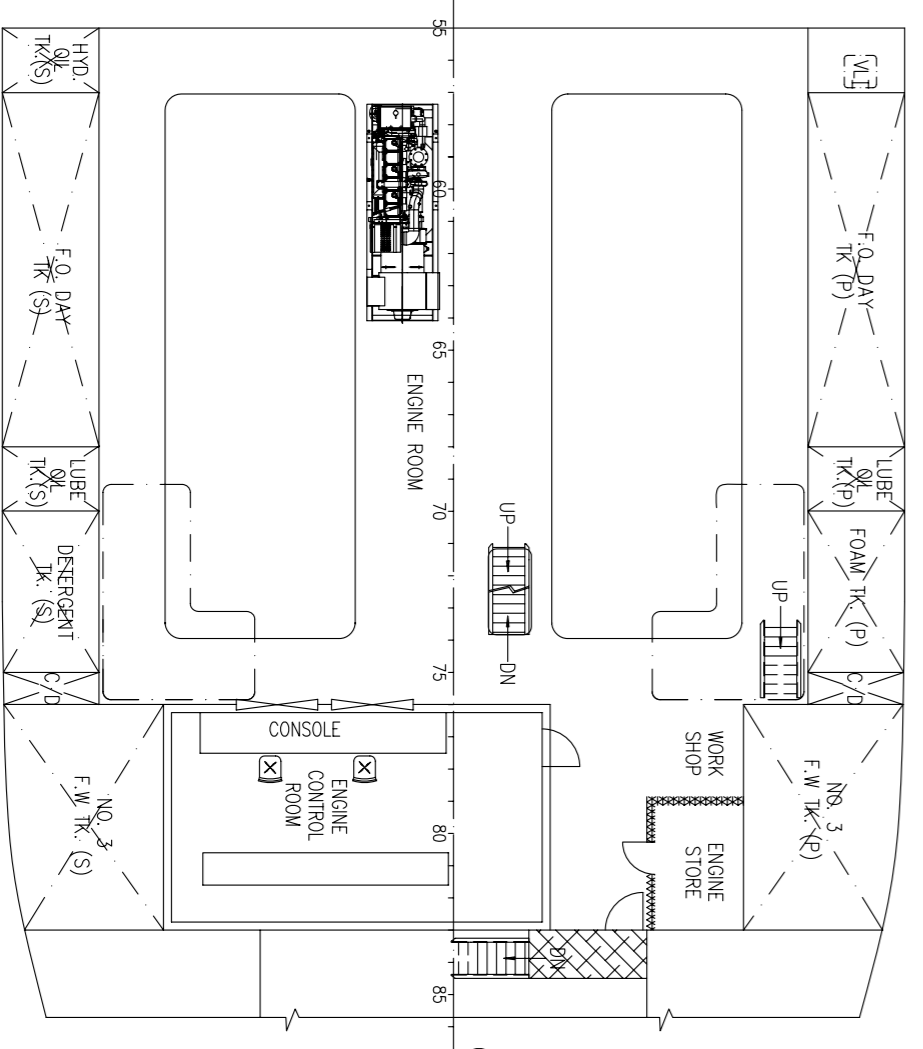
TWEEN DECK PLAN
